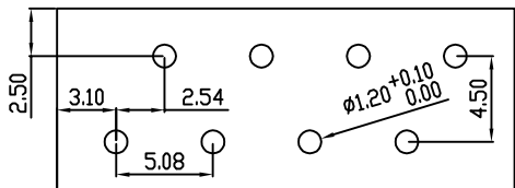
PCB Layout
